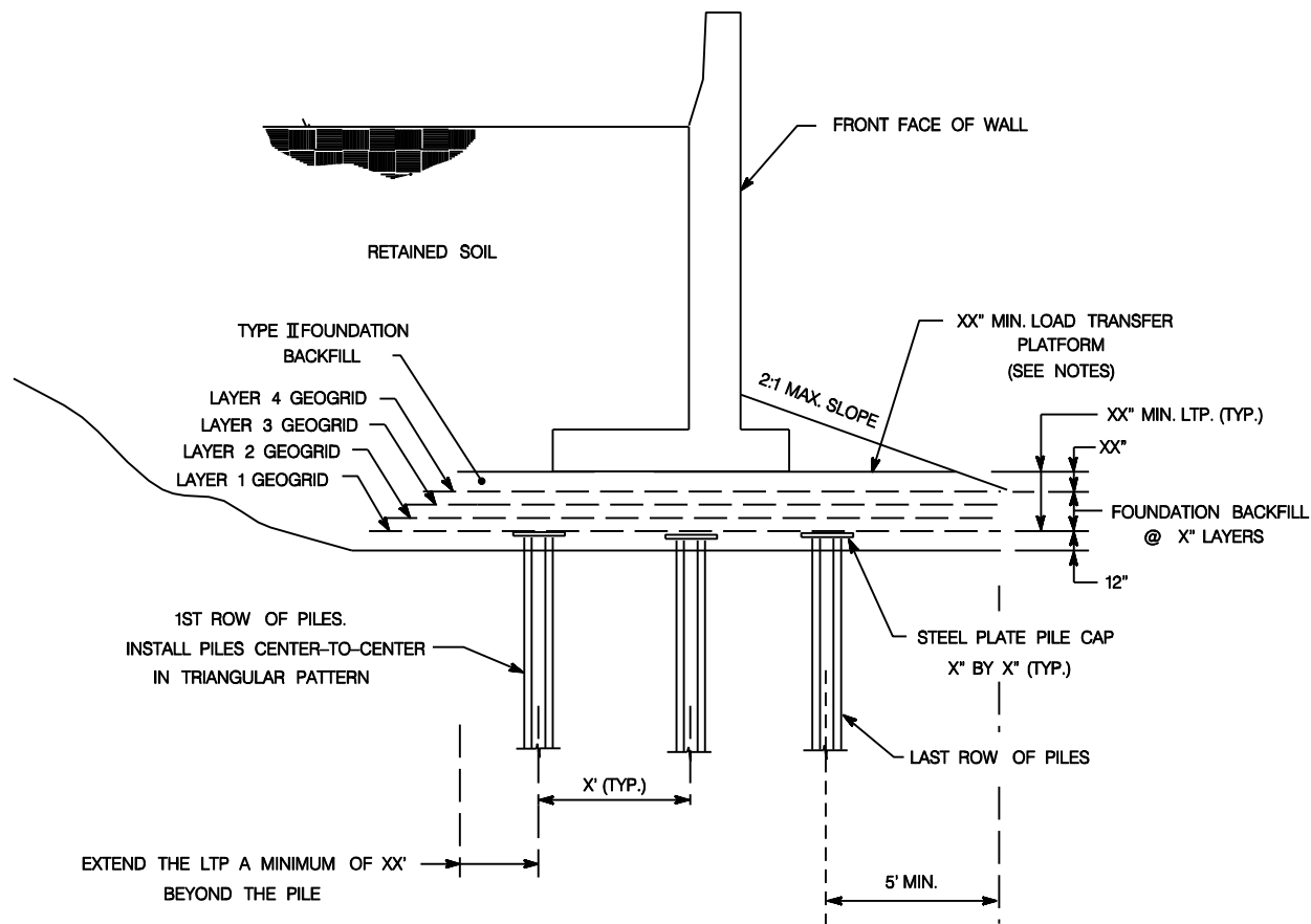
CANTILEVER WALL WITHOUT KEY
